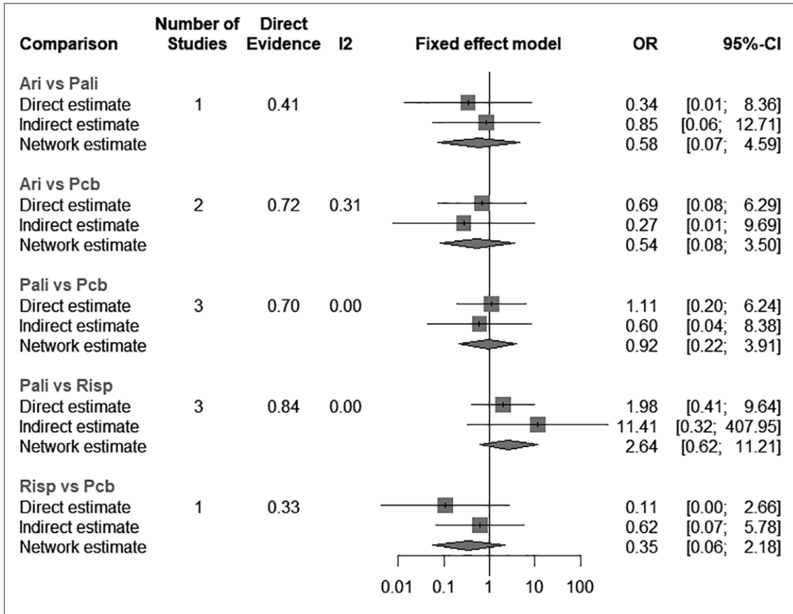
Supplementary Figure 3. Netsplit for deaths. Arip, aripiprazole; Pali, paliperidone; Pcb, placebo; Risp, risperidone; OR, odds ratio; CI, confidence interval.
