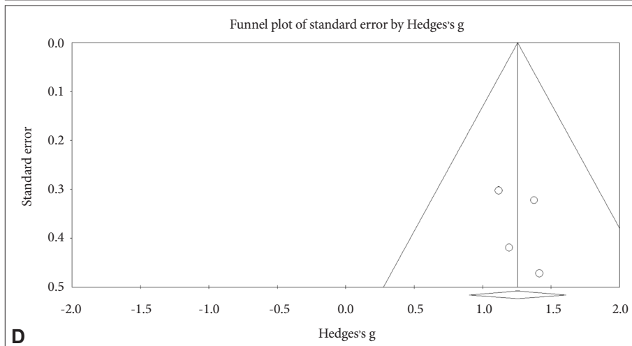
Supplementary Figure 1. Funnel plot of comparison between progressive MCI versus stable MCI participants (A) Any VOI MRI measurement (B) Amyloid PET (C) Hippocampus volume measurement (D) entorhinal cortex volume measurement.
