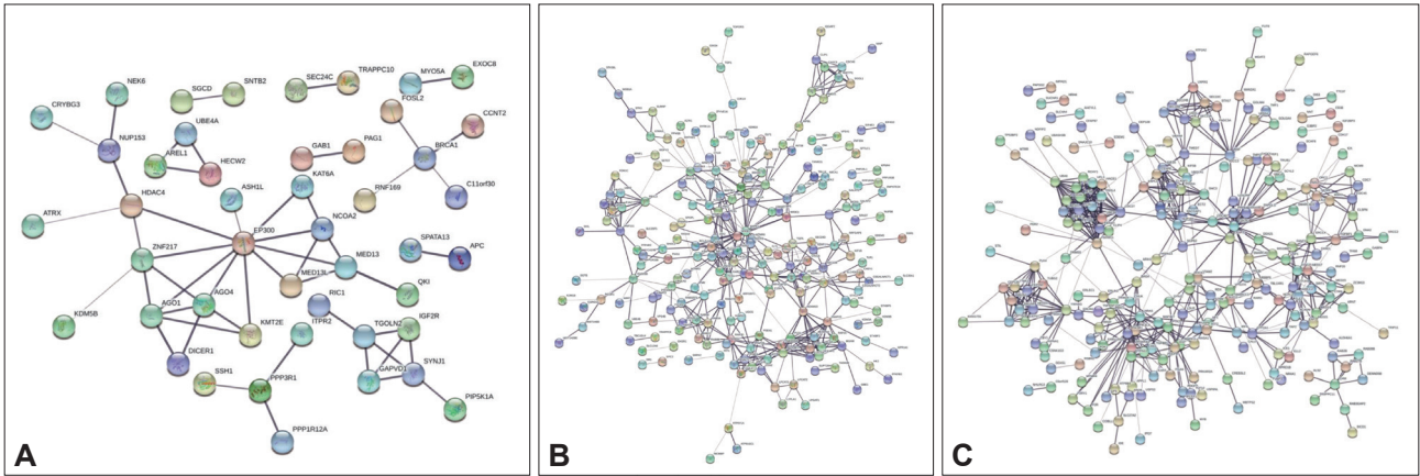
Supplementary Figure 1. Results of PPI network analysis of genes in the three gene modules. A: Black module gene. B: Blue module gene. C: Turquoise module gene.
