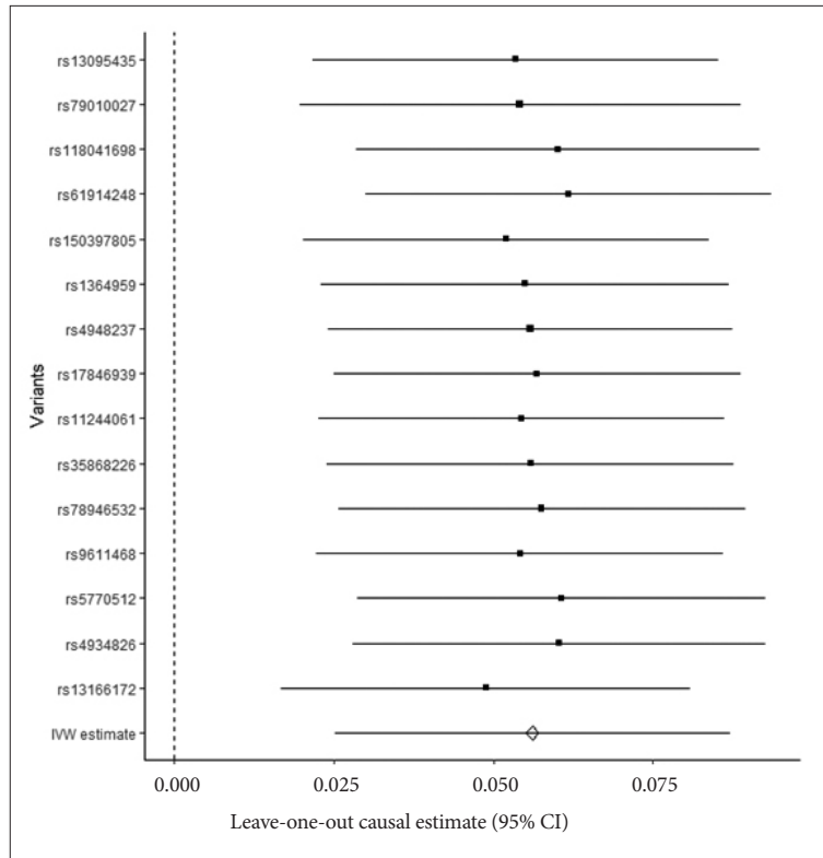
Supplementary Figure 1. Leave-one-out analyses for SNPs associated with left caudal middle frontal surface area (SNPs p < 1 \times 10^{-6} ) \rightarrow CigDay. SNP, single nucleotide polymorphism; CigDay, cigarettes per day; CI, confidence interval.
