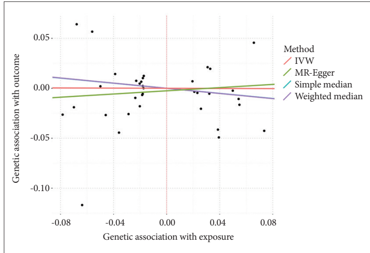
Supplementary Figure 11. Mendelian randomization (MR) plots for AgeSmk (exposure) → Right precentral surface area (outcome); MR-Egger, median, and inverse-variance weighted (IVW) MR analyses. AgeSmk, Age of Initiation of Regular Smoking.
