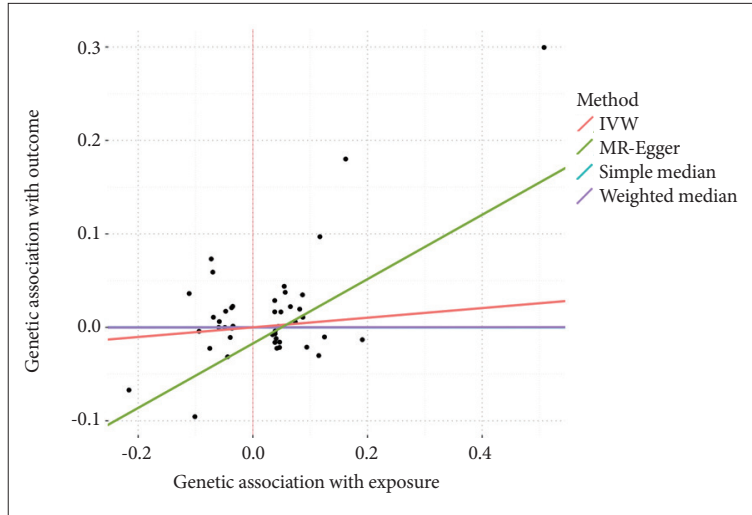
Supplementary Figure 13. Mendelian randomization (MR) plots for (exposure) → left entorhinal thickness SmkCes (outcome); MR-Egger, median, and inverse-variance weighted (IVW) MR analyses. SmkCes, Smoking Cessation.
