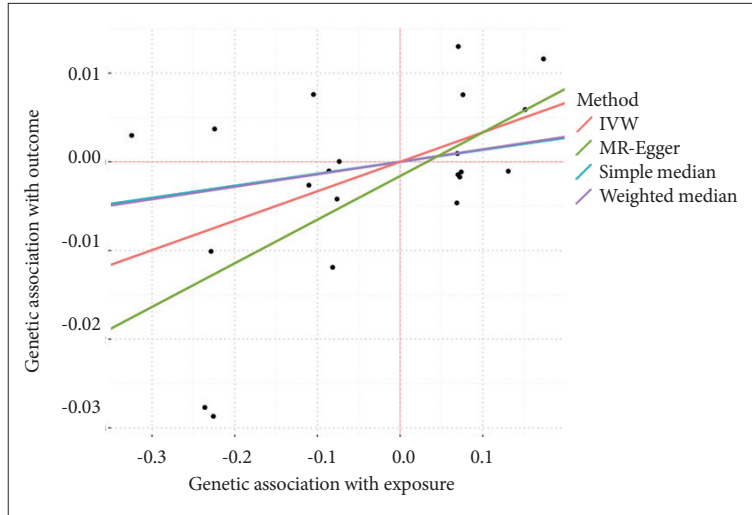
Supplementary Figure 14. Mendelian randomization (MR) plots for Right caudal anterior cingulate thickness (exposure) → AgeSmk (outcome); MR-Egger, median, and inverse-variance weighted (IVW) MR analyses. AgeSmk, Age of Initiation of Regular Smoking.
