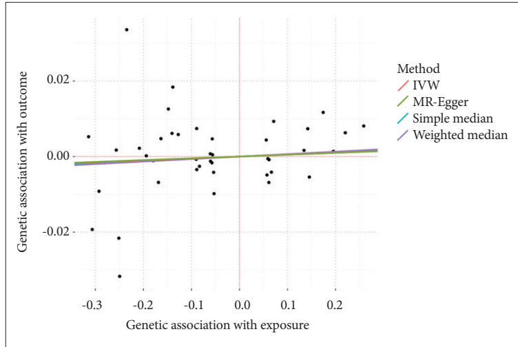
Supplementary Figure 2. Mendelian randomization (MR) plots for Left caudal anterior cingulate surface area (exposure) → AgeSmk (outcome); MR-Egger, median, and inverse-variance weighted (IVW) MR analyses. AgeSmk, Age of Initiation of Regular Smoking.
