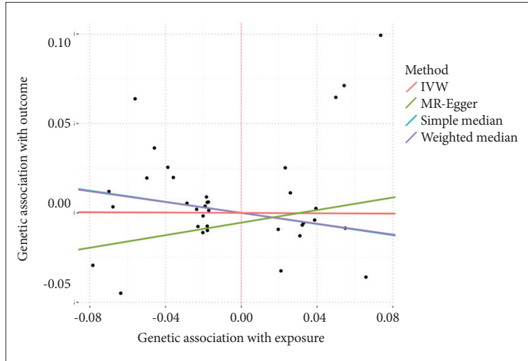
Supplementary Figure 7. Mendelian randomization (MR) plots for AgeSmk (exposure) → Left inferior parietal surface area (outcome); MR-Egger, median, and inverse-variance weighted (IVW) MR analyses. AgeSmk, Age of Initiation of Regular Smoking.
