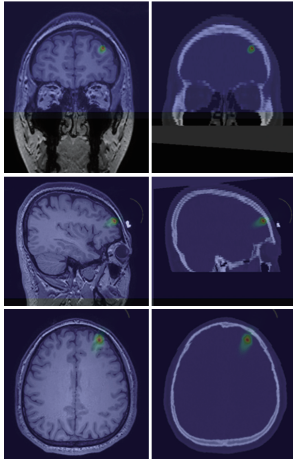
Supplementary Figure 3. An exemplary numerical simulation of acoustic propagation from one individual overlaid on anatomical magnetic resonance imaging. Tri-planar sections are shown at the maximal acoustic intensity.
