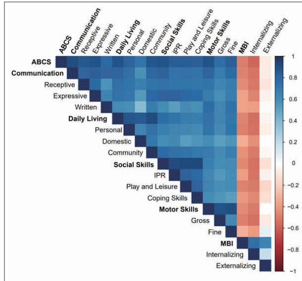
Supplementary Figure 1. Correlation matrix of Korean version of Vineland Adaptive Behavior Scales, Second Edition in developmental disabilities. ABCS, Adaptive Behavior Composite Score; Daily Living, daily living skills; IPR, interpersonal relationships; Play and Leisure, play and leisure time; MBI, Maladaptive Behavior Index; Internalizing, internalizing behaviors; Externalizing, externalizing behaviors.
