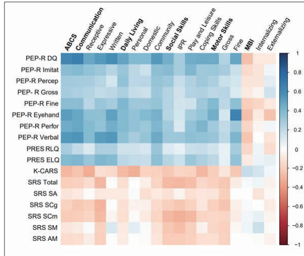
Supplementary Figure 4. Correlation matrix between Korean version of Vineland Adaptive Behavior Scales, Second Edition and the other developmental assessment instruments in typical development. ABCS, Adaptive Behavior Composite Score; Daily Living, daily living skills; IPR, interpersonal relationships; Play and Leisure, play and leisure time; Internalizing, internalizing behaviors; Externalizing, externalizing behaviors; MBI, Maladaptive Behavior Index; PEP-R, Psychoeducational Profile-Revised; DQ, Developmental Quotient; Imitat, Imitation; Percep, perception; Eyehand, eye-hand coordination; Perfor, cognitive performance; Verbal, cognitive verbal; PRES, Preschool Receptive-Expressive Language Scale; RLQ, Receptive Language Quotient; ELQ, Expressive Language Quotient; K-CARS, Korean version of the Childhood Autism Rating Scale; SRS, Social Responsiveness Scale; Total, total score; SA, social awareness; SCg, social cognition; SCm, social communication; SM, social motivation; AM, autistic mannerisms.
